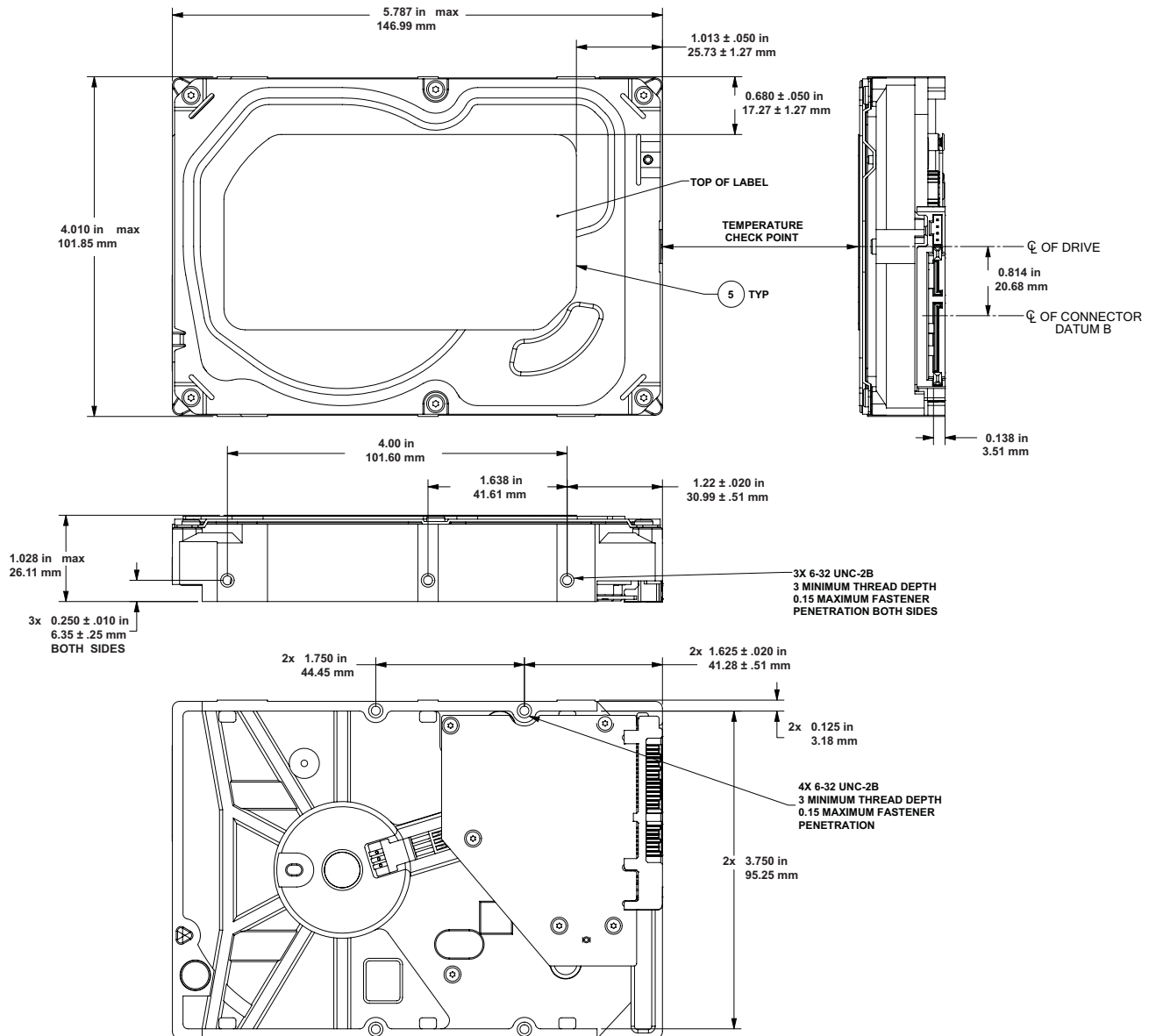
Figure 2 Mounting dimensions (3TB and 4TB)
