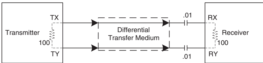
Figure 17. SAS transmitters and receivers
