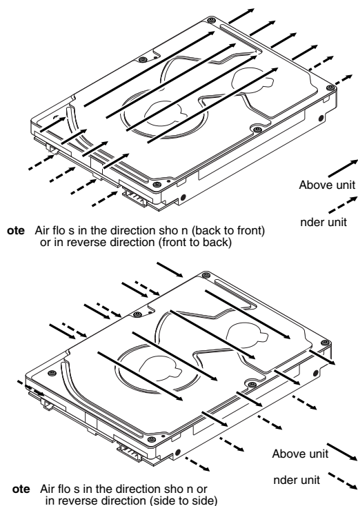
Figure 16. Air flow
