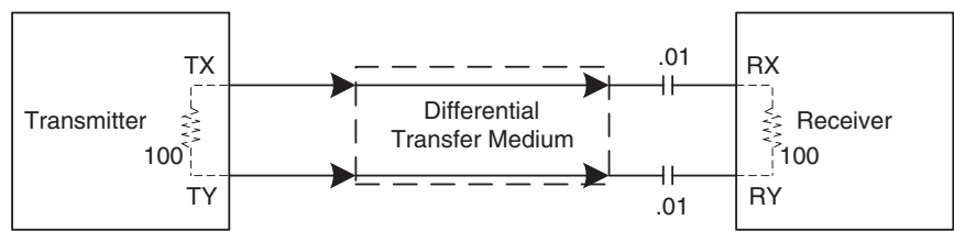
Figure 20. SAS transmitters and receivers
