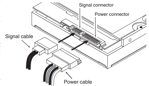
Figure 3. Attaching SATA cabling
