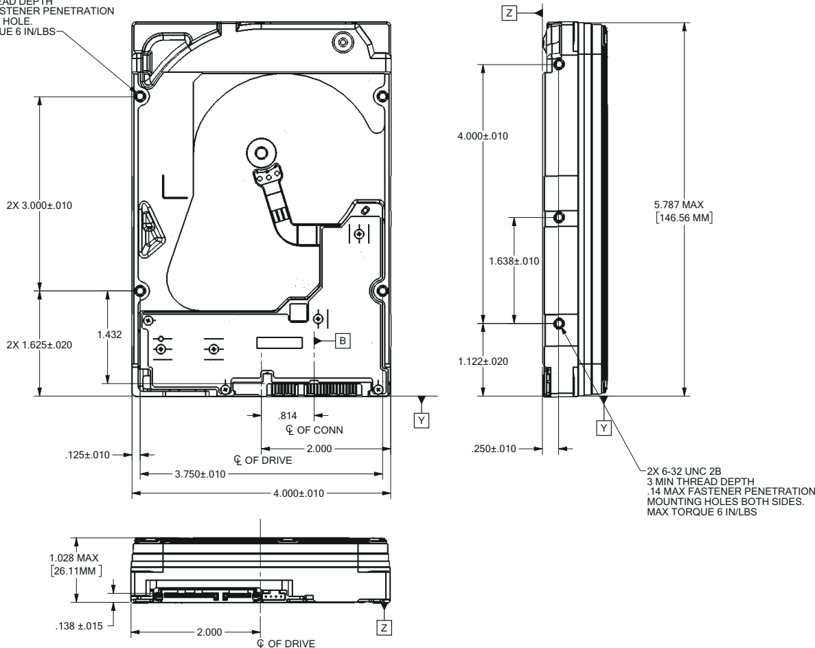
Figure 3. Mounting configuration dimensions
