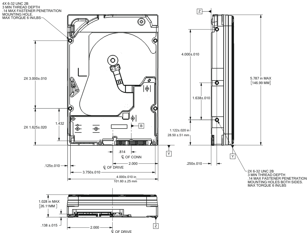
Figure 3. Mounting configuration dimensions
