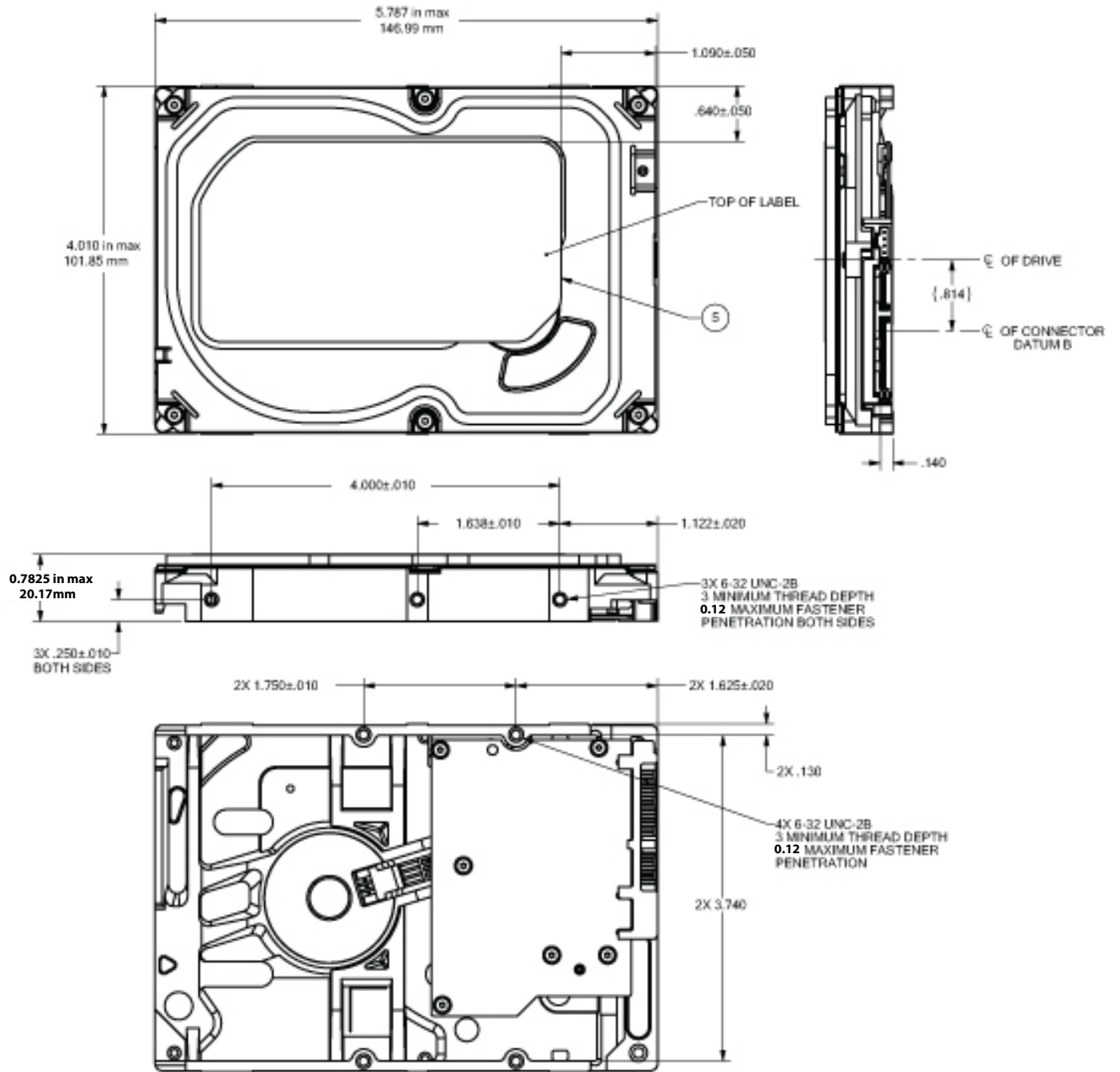
Figure 3 Mounting dimensions (1TB model)
