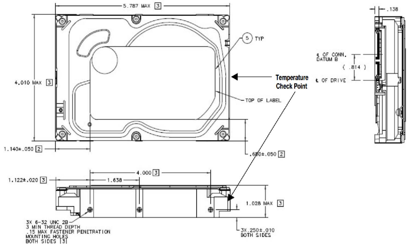
Figure 4 Mounting dimensions
