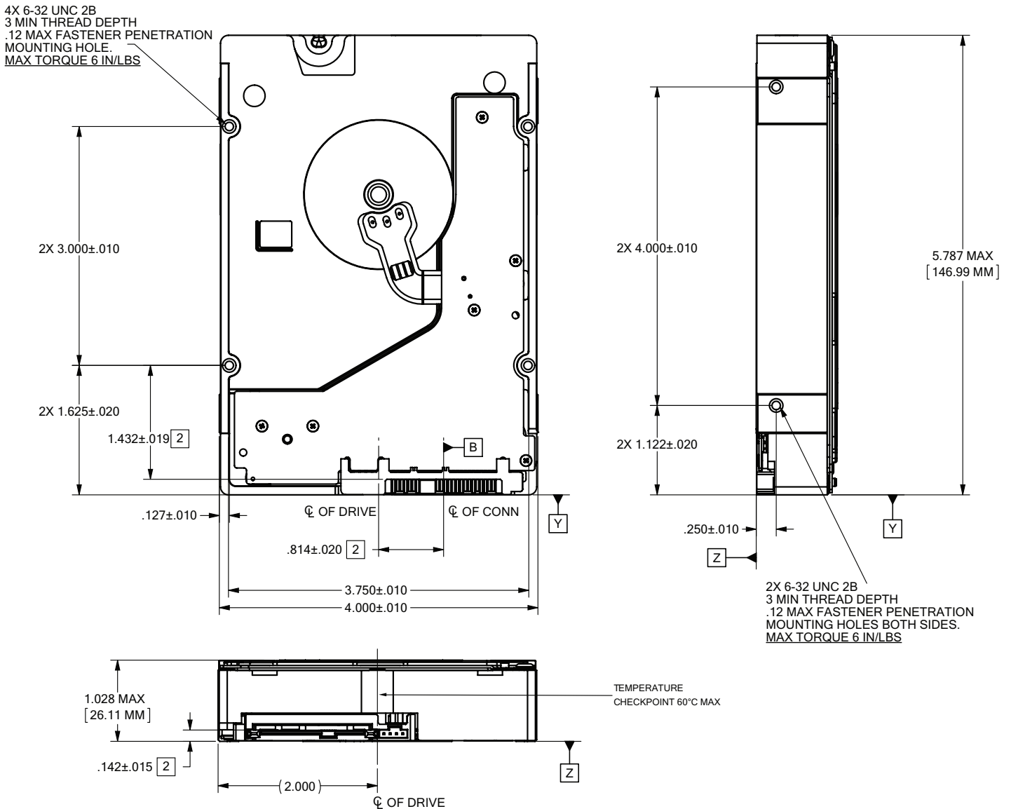
Figure 4. Mounting configuration dimensions (10TB)
