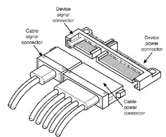
Figure 2. Attaching SATA cabling
