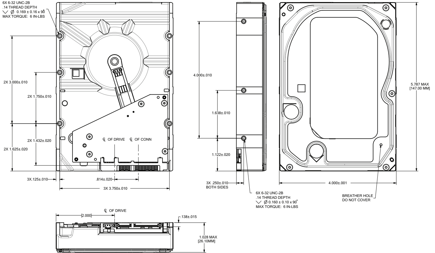
Figure 3. Mounting configuration dimensions 8TB models (Option 1)
