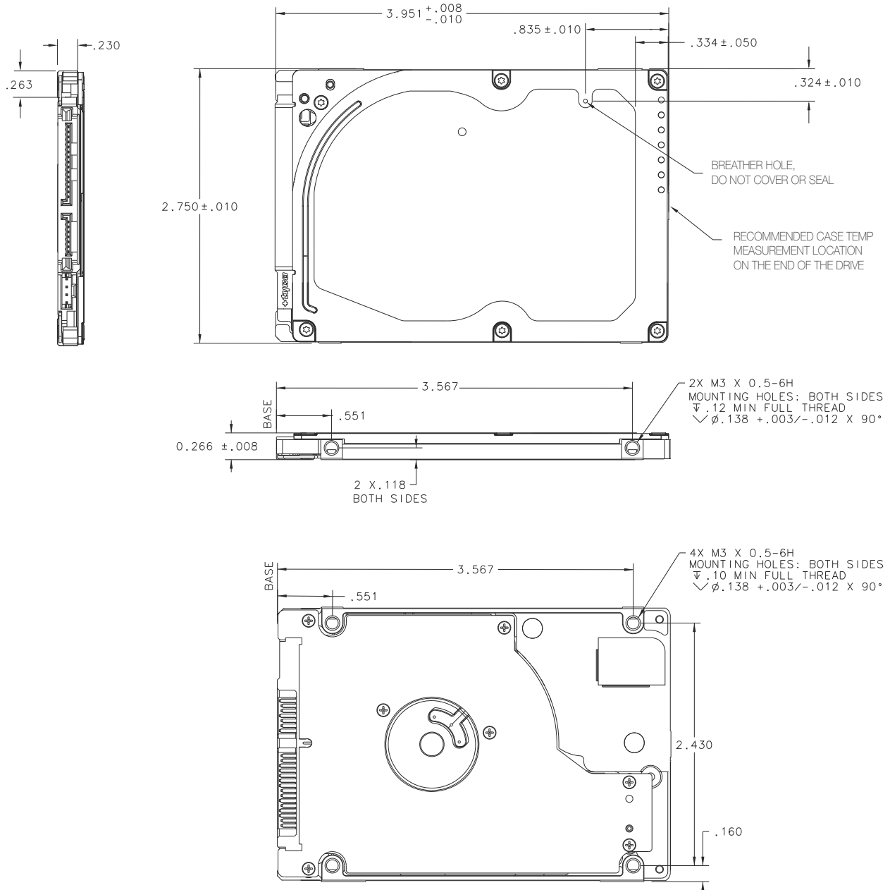
Figure 3 Mounting Dimensions
