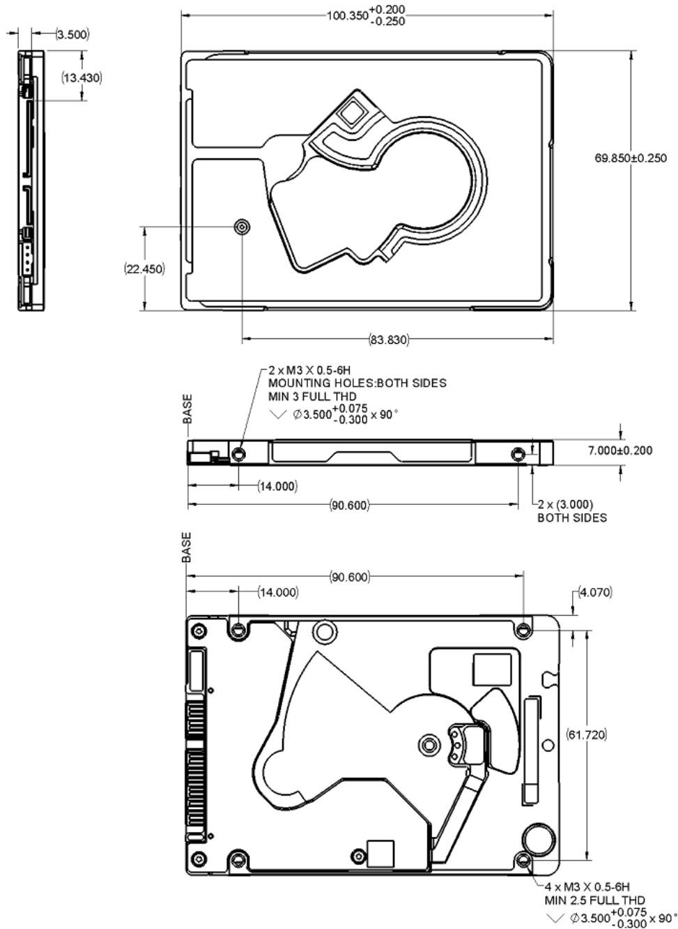
Figure 4 Mounting Dimensions
