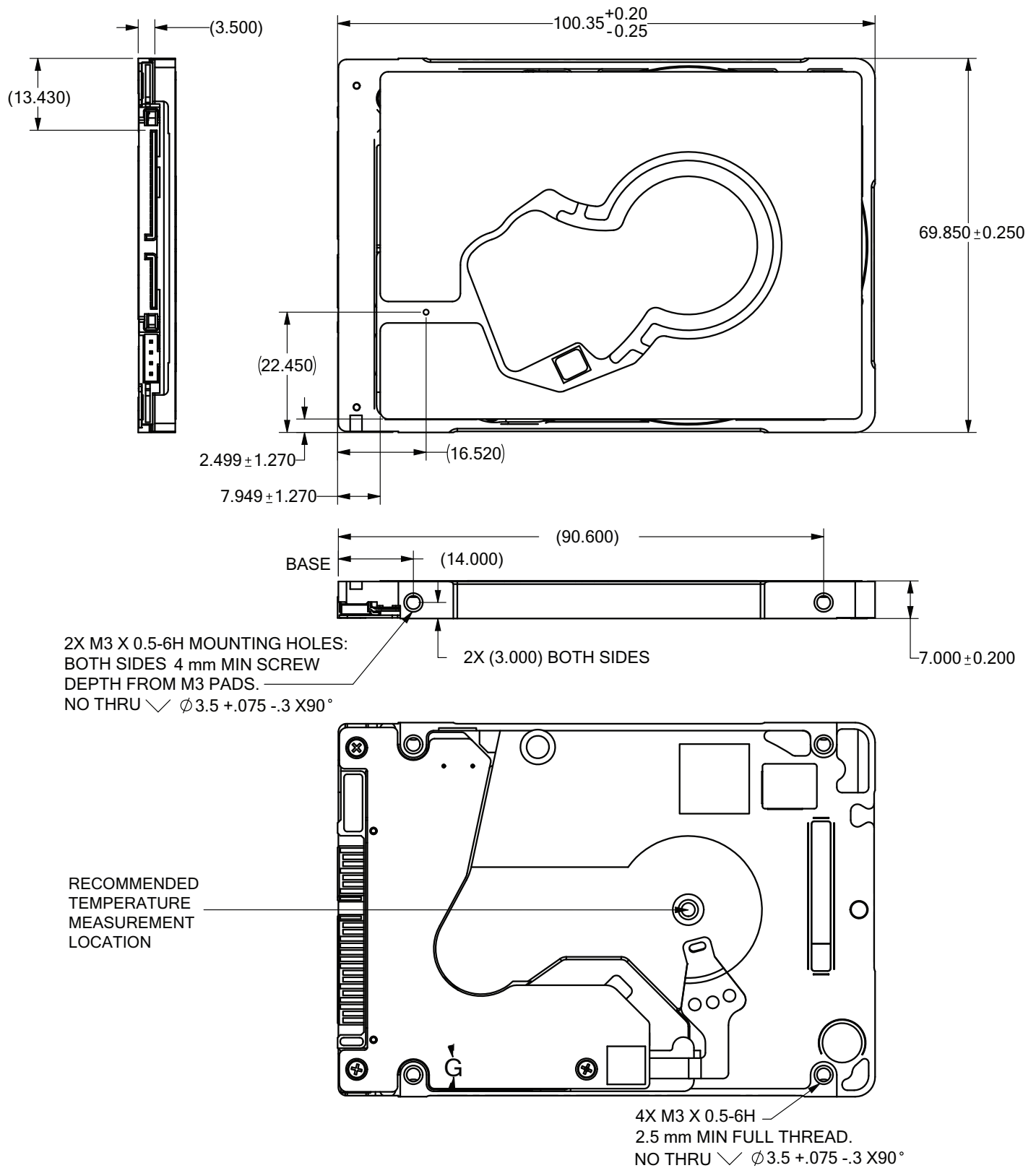
Figure 5 Mounting Dimensions (for 2-disk models)
