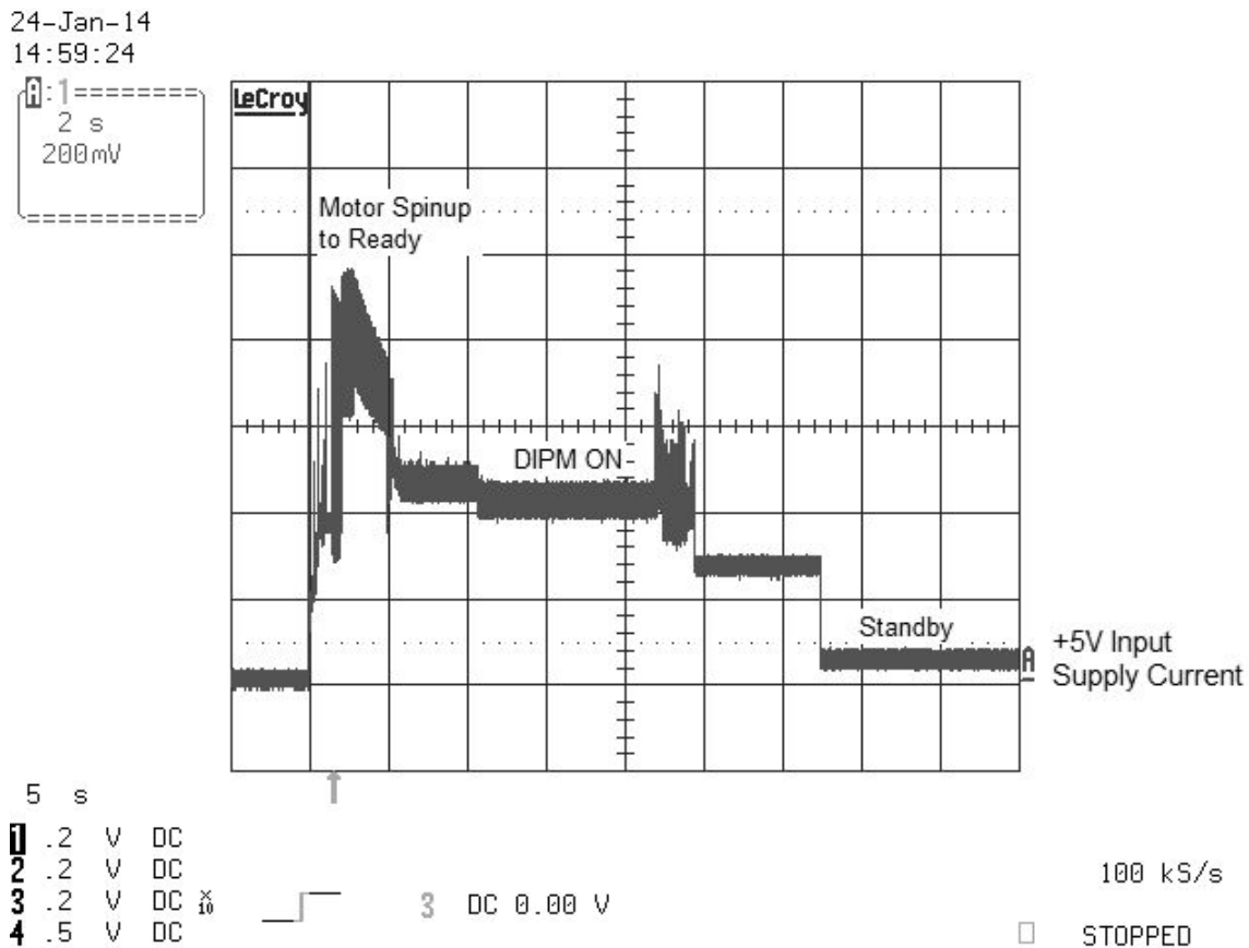
Figure 2 Typical 5V Startup and Operation Current Profile for 16GB models
