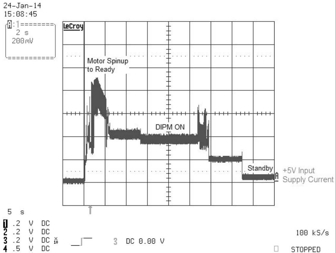
Figure 2 Typical 5V Startup and Operation Current Profile for 16GB models
