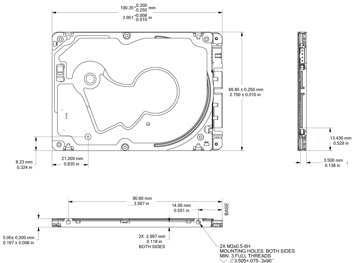
Figure 4 Mounting Dimensions (for standard models)
