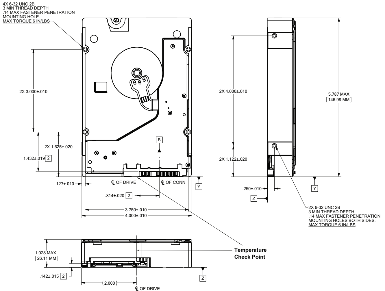
Figure 3 Mounting dimensions
