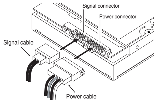
Figure 2 Attaching SATA cabling
