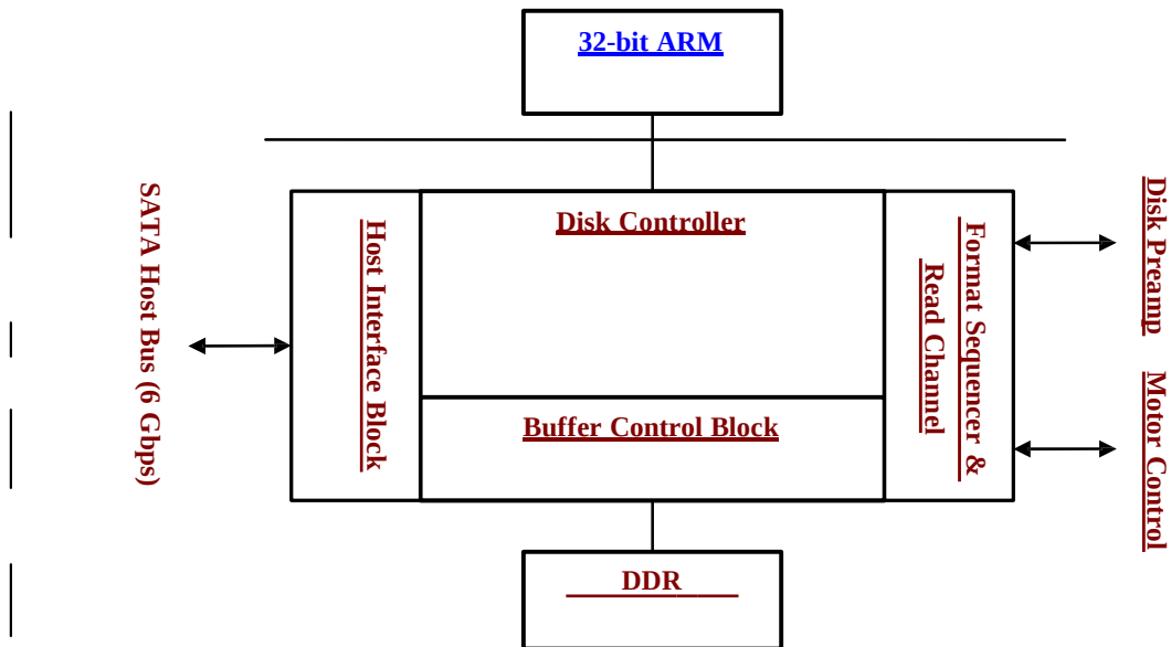
Figure 5-2: Spinpoint M8 Functional Block Diagram
